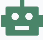
Artificial intelligence
